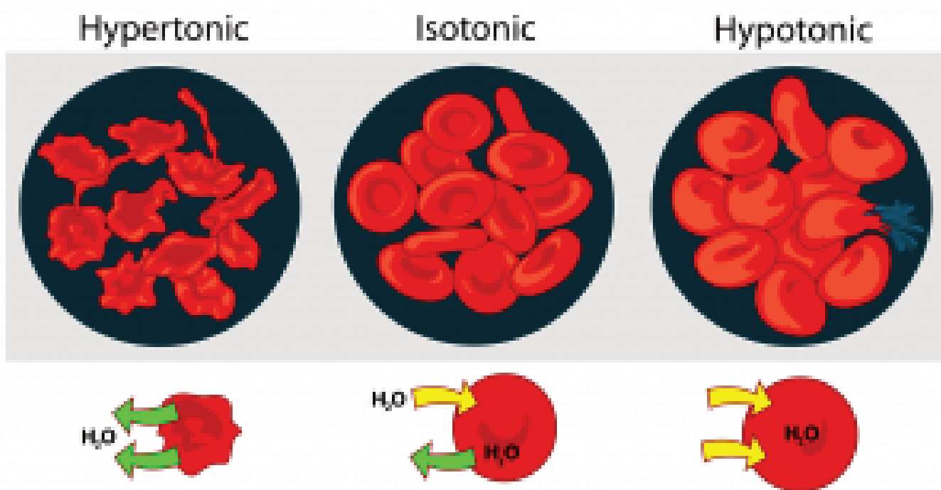
Figure 3.3 Osmoregulation
